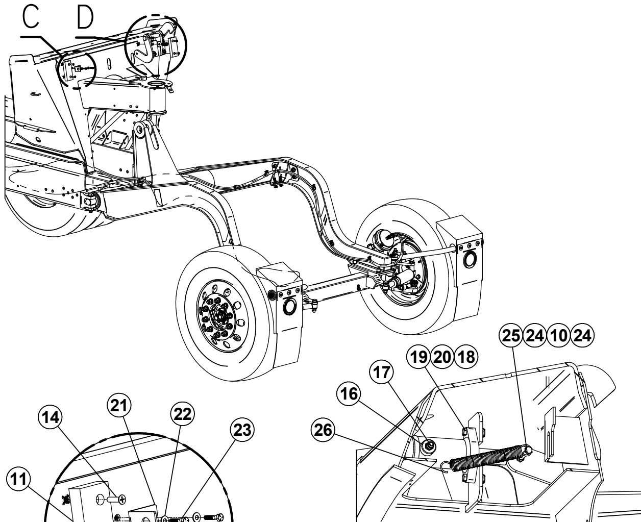
SECTION VIEW INSIDE REAR PEDESTAL
